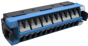
360 Distribution Adapter Pack, Singlemode, 24 LC/UPC with internal shutters
